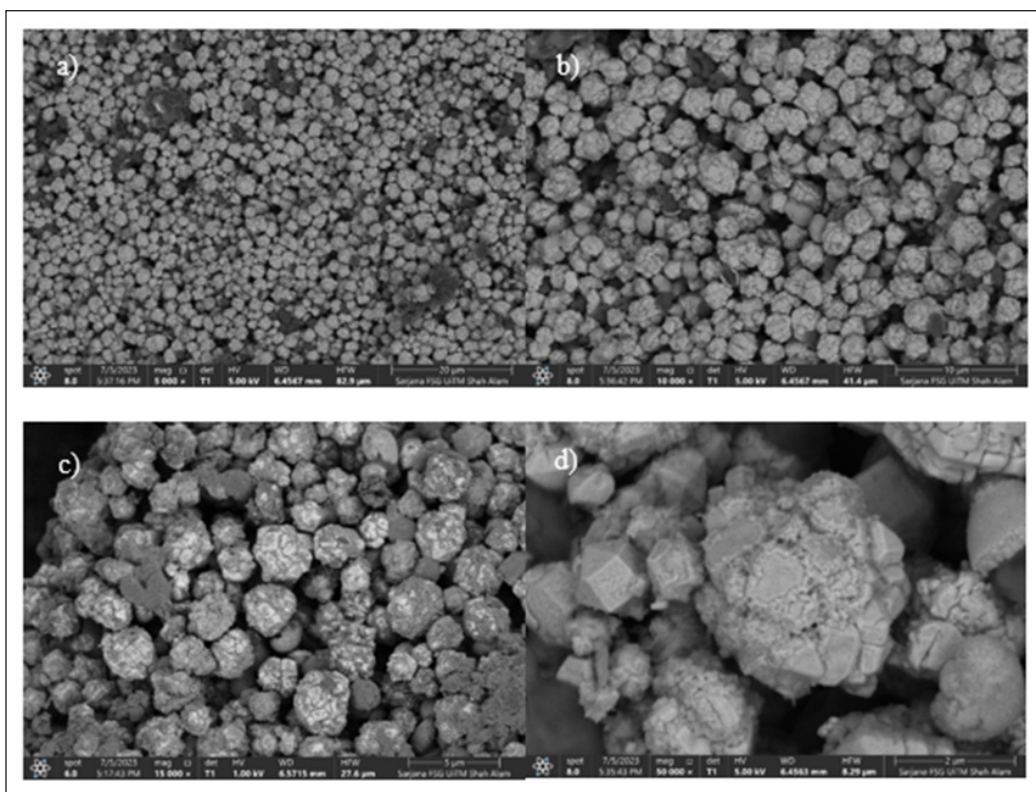
Figure 5. The morphological surface structure of synthesised copper nanoparticles using Ananas comosus leaf extract using (a) 1000 x, (b) 10000 x, (c) 15000 x, and (d) 50000 x magnification of Field Emission Scanning Electron Microscopy (FESEM)
